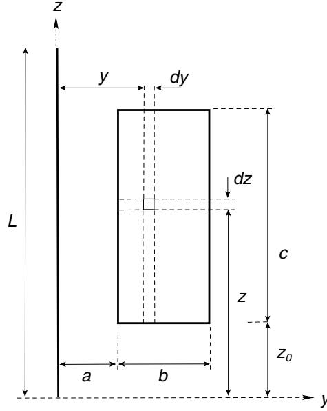
Figure 1: Configuration of loop parallel to straight wire.
