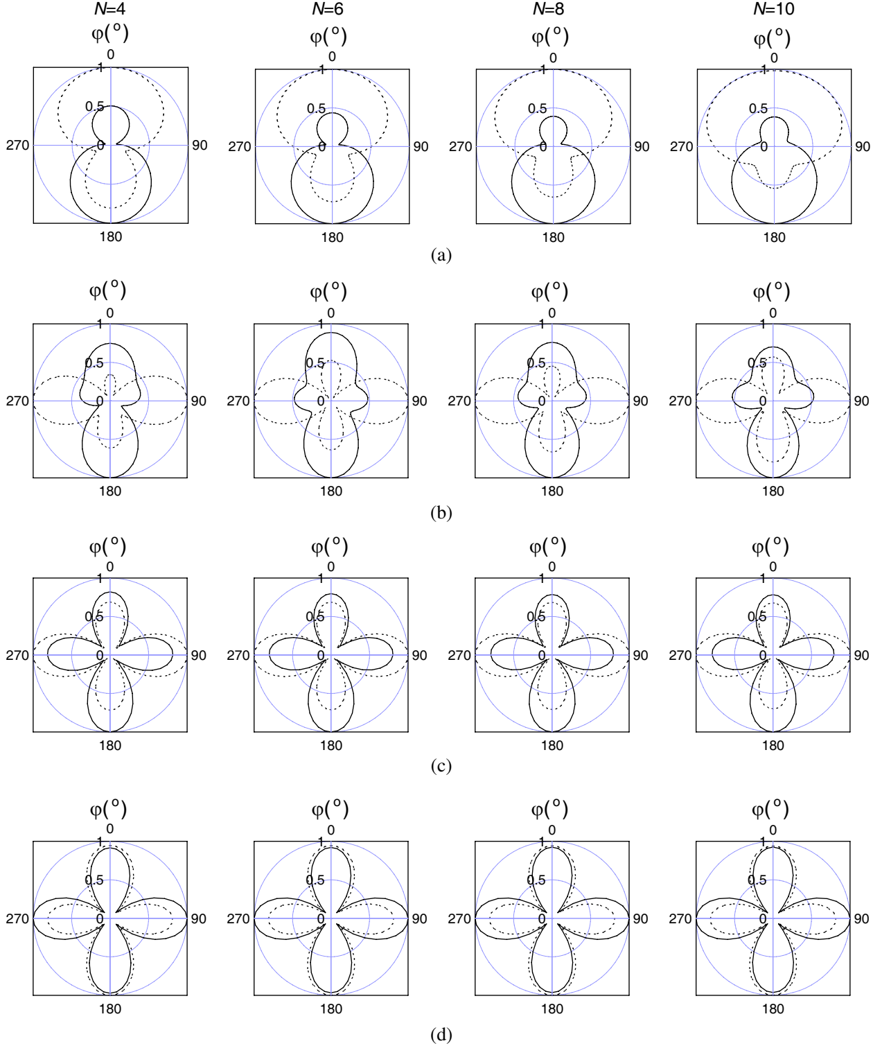
Figure 4: Electric field patterns on the azimuthal plane: —: E_\theta ; - - - - -: E_\phi . (a) S_\lambda = 0.1 , (b) S_\lambda = 1.0 , (c) S_\lambda = 1.4 , (d) S_\lambda = 1.8 .
