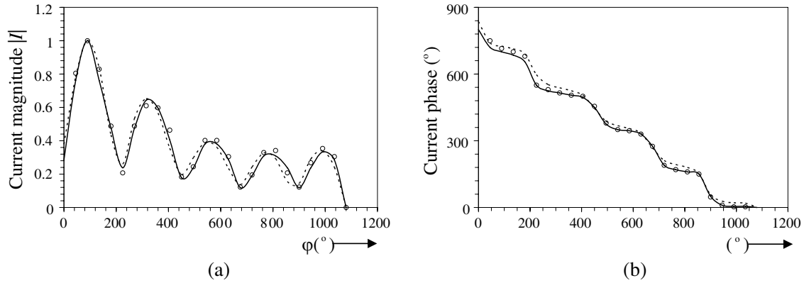
Figure 2: Comparison of current magnitude and phase of a centre-fed helical antenna at 500 MHz: — — —: MoM; ———: Chen's theory and \circ \circ \circ \circ : Experimental results at 500 MHz of Figure 6(a) [3].
