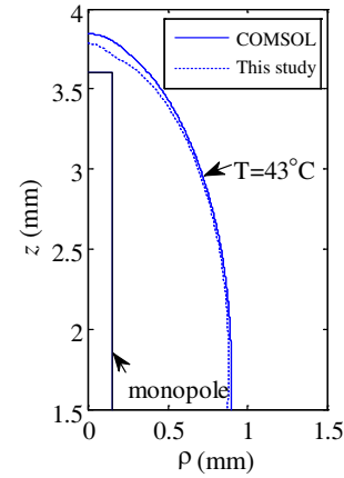
Figure 7: Comparison of temperature contour at 43°C with COMSOL simulation.
