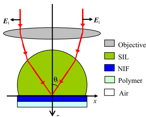
Figure 1: Schematic diagram of the focusing system in the near-field optical storage with an aplanatic solid immersion lens.
