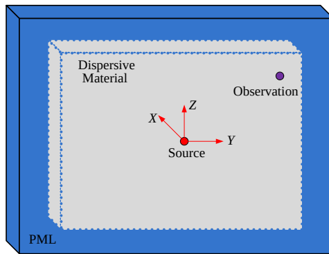
Figure 1: The FDTD grid geometry in this simulation.
