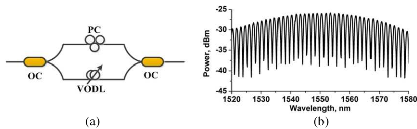
Figure 1: (a) The structure of an FMZI and (b) the sliced spectrum of the BOS after the FMZI.
