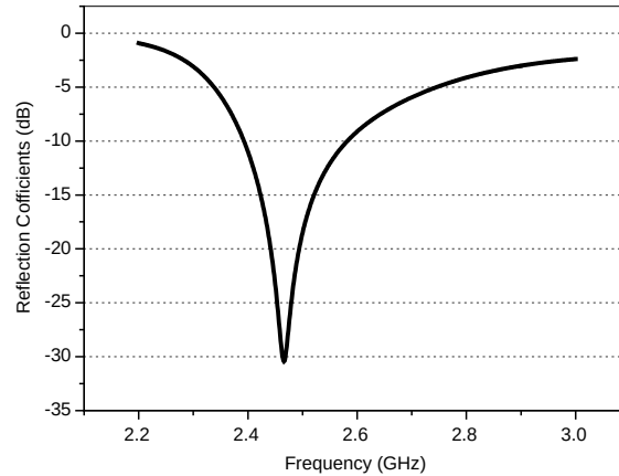
Figure 2: Simulated reflection coefficients of the proposed antenna.
