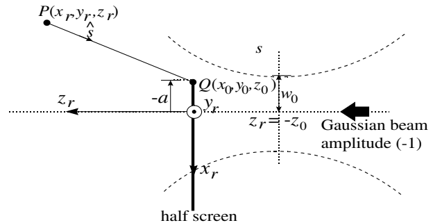
Figure 2: Mirror-symmetric geometry for determining the backward-scattered field.
