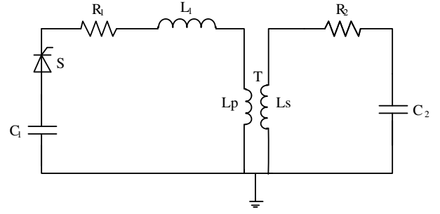
Figure 2: The discharge circuit of pulse transformer.
