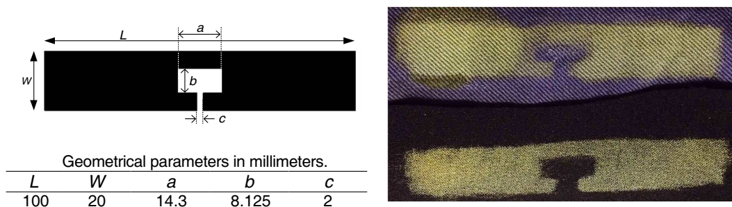
Figure 1: Antenna geometry and samples of brush-painted antennas.
