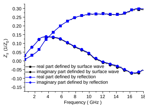
Figure 4: Surface impedance defined by surface wave characteristic and by the reflection coefficient of RAM A backed with a perfect electric conductor (PEC) plate, and its thickness is 0.5 mm.
