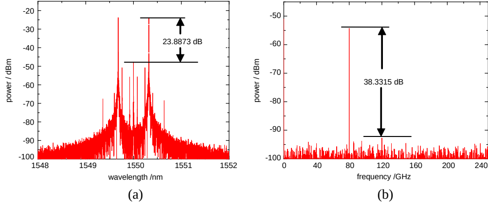
Figure 3: The simulated 80 GHz mm-wave signal generation for ER = 30 dB. (a) The output optical spectrum of the integrated MZM; and (b) the generated RF spectrum.
