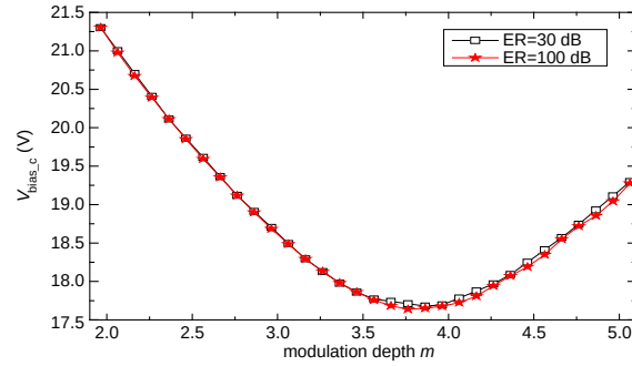
Figure 5: The best V_{bias,c} of MZM-c versus different modulation depths m .
