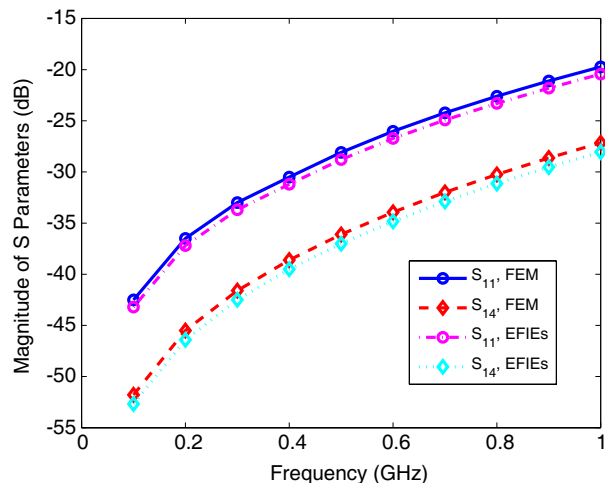
Figure 2: S parameter for the interconnect and packaging structure including a signal line and a one-layer dielectric substrate. The geometry is defined with l = 10.0 , w = 5.0 , d = 0.1 , s = 0.2 , t = 0.05 , and h = 0.3 , all in millimeters, and the substrate has a relative permittivity \epsilon_r = 4.0 .
