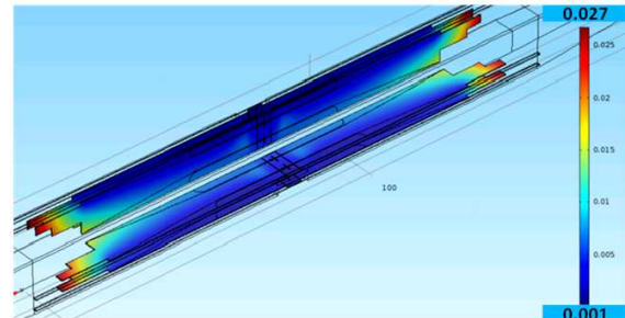
Figure 10: Total displacement (mm) in the Squarax SPC volume, due to heat generation inside the MMIC SSPA's.
