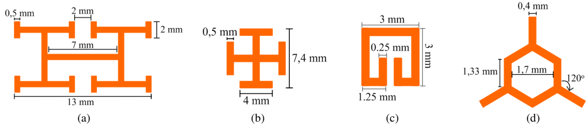
Figure 1: (a) Unitary fractal cell, (b) unitary JCP cell, (c) unitary CLL cell, (d) tripole array.
