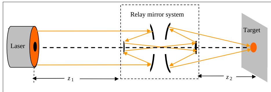
Figure 1: Configuration for beams through a relay mirror system.
