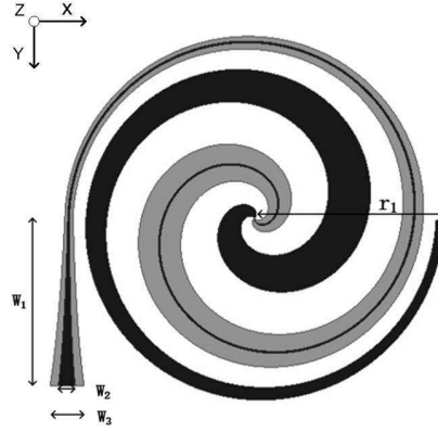
Figure 2: The geometry of the proposed antenna. Metal on the front side (black) and metal on the back side (gray).
