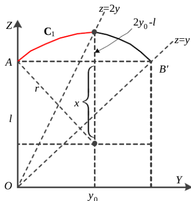
Figure 4: Panel geometry of circular arc.
