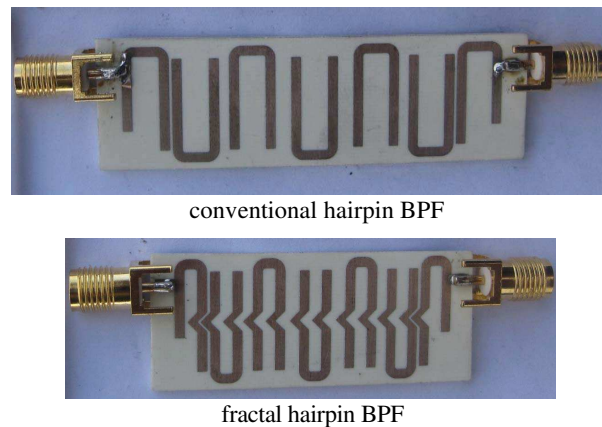
Figure 5: Pictures of both realized hairpin band-pass filters.
