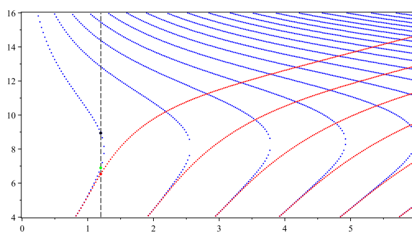
Figure 3: Case 1(b). Marked eigenvalues: \gamma \approx 2.554 (red dot), \gamma \approx 2.624 (green dot), and \gamma \approx 3.988 (black dot).
