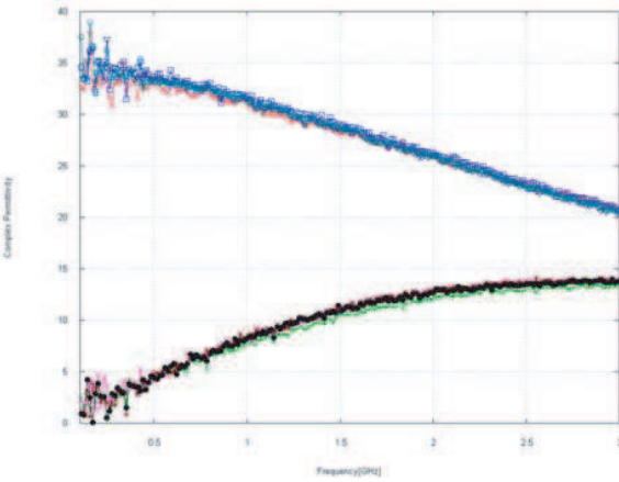
Figure 8: Frequency characteristics of complex permittivity (methanol).
