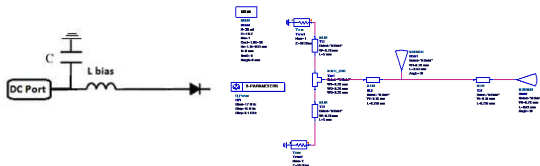
Figure 9: The biased circuit for diode.
