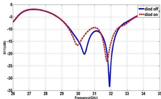
Figure 11: The S parameter of antenna.
