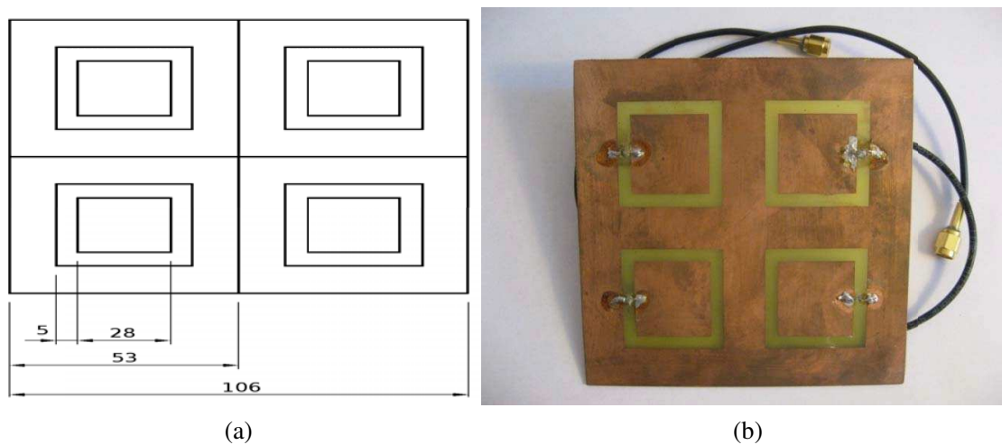
Figure 4: Composition of (a) four rectangular shaped slot planar applicators scheme, (b) final designed model.
