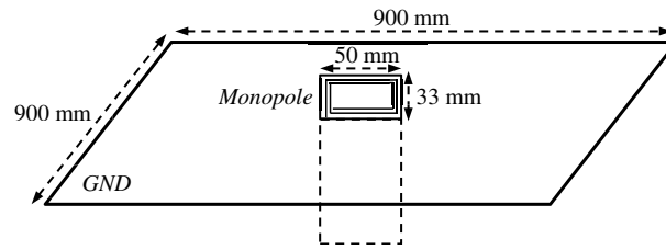
Figure 3: The FM antenna on large ground plane.
