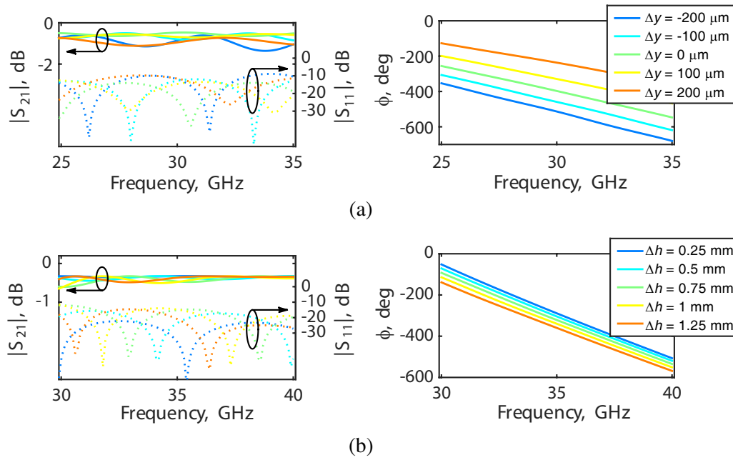
Figure 2: Simulated scattering parameters for different states of reconfiguration. (a) Concept of Fig. 1(a): L_{PS} = 10 mm, L_{tr} = 200 \mu\text{m} , substrate with \epsilon_r = 9.8 and \tan \delta = 0.002 (e.g., Rogers TMM10i). The compliant connections are modeled as a resistive sheet with R_S = 30 \Omega/\square [14]. (b) Concept of Fig. 1(b): L_{PS} = 20 mm, L_{tp} = 5 mm. A conductivity \sigma = 2.9 \times 10^7 S/m is considered for all metallic parts, and actuators are completely shielded from the EM active area.
