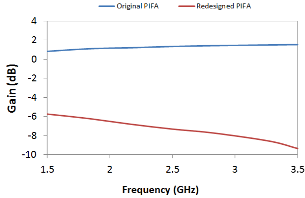
Figure 5: Antenna gain for the (a) original and (b) redesigned meandered PIFA antenna.
