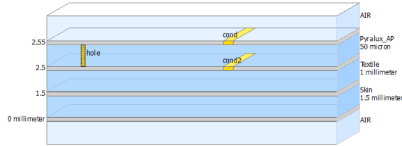
Figure 1: Substrate definition including F-PCB, textile and skin effects.
