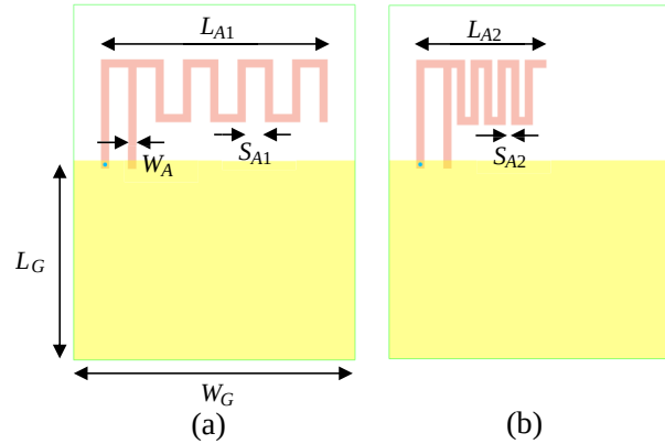
Figure 2: Geometry of the (a) original and (b) redesigned meandered PIFA antenna.
