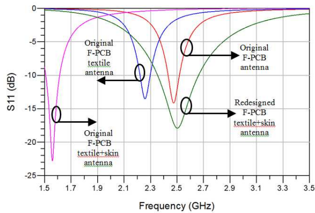
Figure 3: Return loss of the original and redesigned PIFA antennas.
