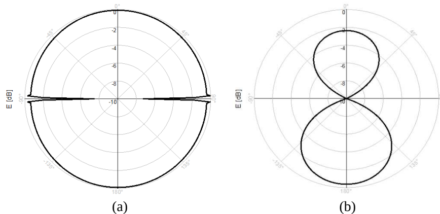
Figure 4: Normalized radiation pattern for the maximum radiation level case at 2.45 GHz for the (a) original ( \phi = 141^\circ ) and (b) redesigned meandered PIFA antenna ( \phi = 177^\circ ).
