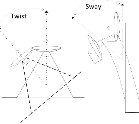
Figure 3: The motion of the antenna mast as twist and sway.
