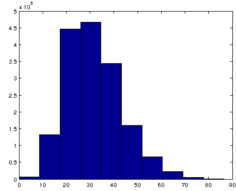
Figure 5: The PDF of capacity in distributed MIMO.
