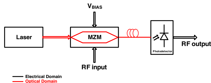
Figure 1: Optical link.
