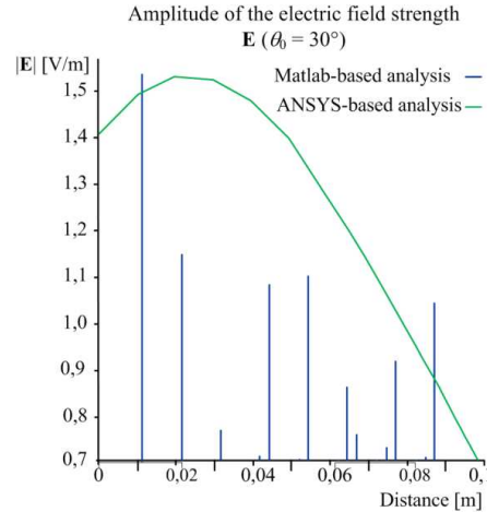
Figure 3: The diagram of the distribution of the electric field strength \mathbf{E} : for \theta_0 = 30^\circ , on the surface of the material, and in the plane of incidence.
