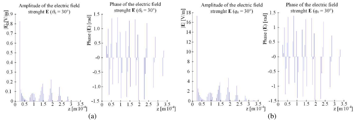
Figure 4: The strength of the electric component of the TE wave on a layered medium for d = \lambda \cdot 100 and (a) t = T , (b) t = 20 \cdot T ( f = 700 THz).
