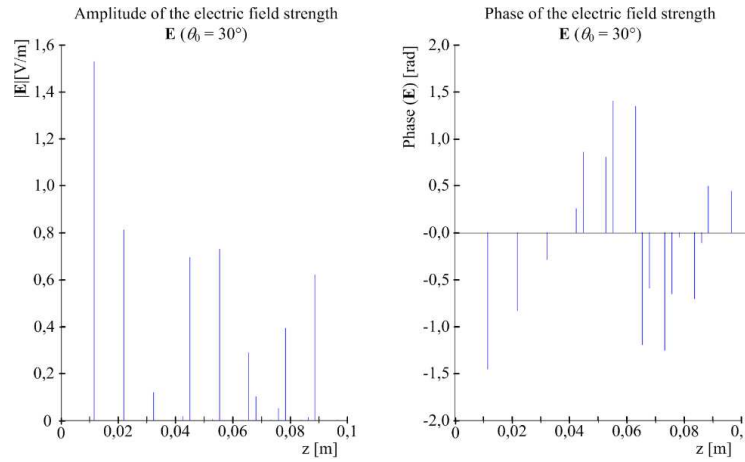
Figure 2: The strength of the electric component of the TE wave on a layered medium at the angle \theta_0 = 30^\circ .
