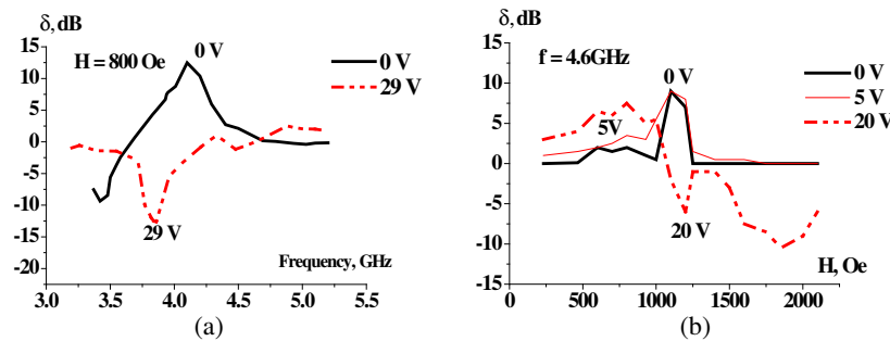
Figure 3: (a) Dependences of nonreciprocity \delta , \text{dB} = T(H_-) - T(H_+) on frequency in metastructure ferrite plate/varactor loaded split Butterfly dipole under H = 800 Oe at bias voltage V_{DC} = 0 (sign of \delta is positive) and V_{DC} = 29 V (sign of \delta is negative). (b) Dependences of \delta on H -field value in metastructure ferrite plate/chains of varactor loaded double split rings under f = 4.6 GHz at bias voltage V_{DC} = 0, 5, 20 V.
