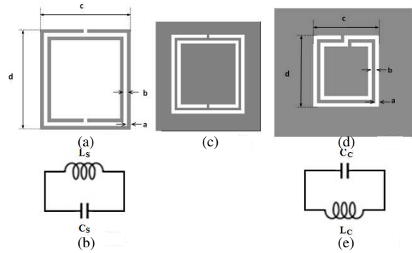
Figure 2: Sub-wavelength particles dimensions: a = b = 0.2\text{ mm} for all the particles. ISM: c = 5\text{ mm} , d = 5.5\text{--}5.8\text{ mm} . GSM: c = 3.7\text{ mm} , d = 4\text{ mm} . RFID: c = 5.5\text{--}5.9\text{ mm} , d = 7.5\text{ mm} .
