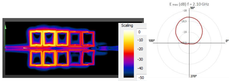
Figure 6: Simulated RMS values for E near-field and normalized radiation pattern at 2.10 GHz.
