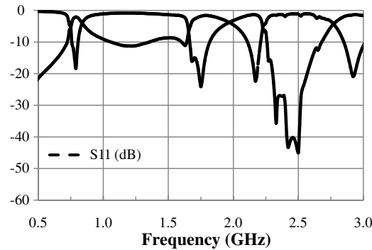
Figure 3: Experimentally measured frequency responses of the insertion losses ( S_{21} ) and return losses ( S_{11} ).
