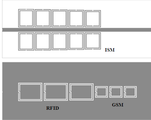
Figure 1: Topology of the designed multiband microstrip EMI filter. (a) Top layer with microstrip line and the SRRs designed at 2.45 GHz. (b) Bottom layer with CSRs etched in the ground metal tuned at 900 MHz and 1.8 GHz, respectively. Metallization zones are depicted in grey.
