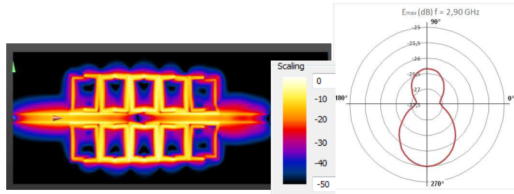
Figure 8: Simulated RMS values for E near-field and normalized radiation pattern at 2.90 GHz.
