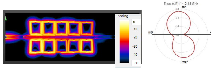
Figure 7: Simulated RMS values for E near-field and normalized radiation pattern at 2.43 GHz.
