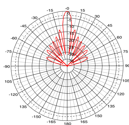
Figure 6: Electric field pattern for 10 elements.
