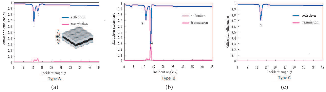
Figure 2: The (0, 0)-th order reflection and transmission efficiency for 3-layered doubly periodic gratings (a) e_{\text{Ag}} = e_{\text{SiO}_2} = 27.8 \text{ nm} ; (b) e_{\text{Ag}} = 27.8 \text{ nm} , e_{\text{SiO}_2} = 278 \text{ nm} ; and (c) e_{\text{Ag}} = 278 \text{ nm} , e_{\text{SiO}_2} = 27.8 \text{ nm} .
