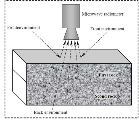
Figure 2: Microwave radiation of two-layer rock.
