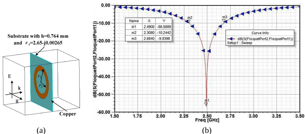
Figure 1: Schematic structure and resonant response of a circular loop with r_1 = 27 mm and r_2 = 19.2 mm. (a) Schematic Structure. (b) Simulated S_{21} .
