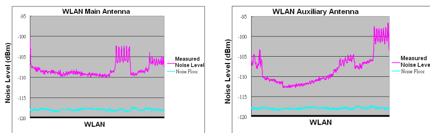
Figure 11: EMI noise power received by main and auxiliary antennas from S3's SSD.
