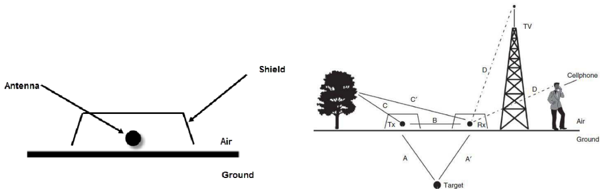
Figure 1: A shielded ground penetrating radar (GPR) antenna.
