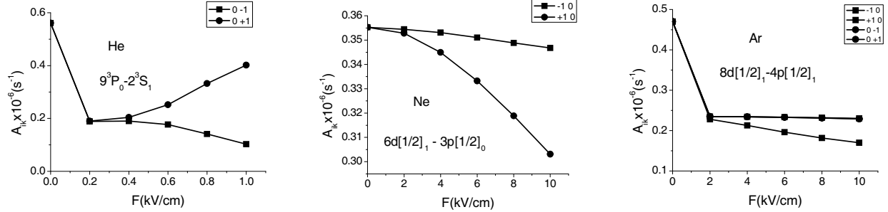
Figure 1: F -dependence of transition probabilities for states with J, J' = 0, 1 ( \omega = 100 \text{ MHz} ).
