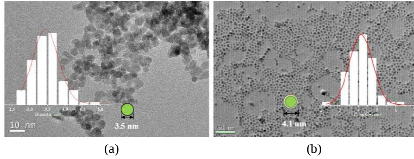
Figure 1: (a) TEM of \text{ZrO}_2:20\%\text{Yb}^{3+}, 2\%\text{Er}^{3+} (core) and histogram of the size distribution (inset); (b) TEM of \text{ZrO}_2:20\%\text{Yb}^{3+}, 2\%\text{Er}^{3+}@\text{NaYF}_4:2\%\text{Yb}^{3+} (core-shell) and histogram of the size distribution (inset).
