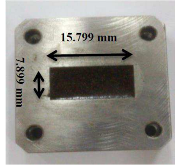
Figure 2: Ku-Band sample holder fit with RHCNTs sample.
