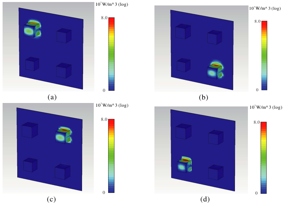
Figure 5: The distribution of the power loss density of the MA at resonance frequencies corresponding to the four different geometrical parameters: (a) at 7.31 GHz, a = 2.7 mm; (b) at 7.58 GHz, a = 2.6 mm; (c) at 7.90 GHz, a = 2.5 mm; (d) at 8.19 GHz, a = 2.4 mm.
