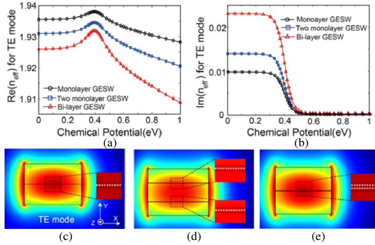
Figure 5: (a) \text{Re}(n_{\text{eff}}) with chemical potential variation for monolayer, two separated monolayer, and bi-layer GESW; (b) \text{Im}(n_{\text{eff}}) with chemical potential variation for monolayer, two separated monolayer, and bi-layer GESW; (c) (d) and (e) represent the electric field distribution for TE polarization mode of monolayer, two separated monolayer, and bi-layer GESW under chemical potential of 0 eV, respectively.
