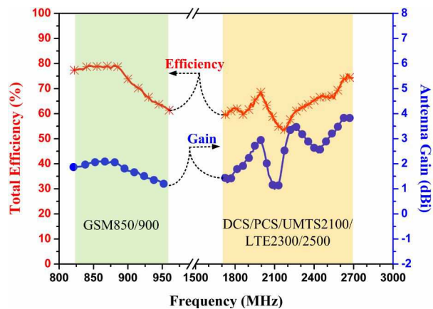
Figure 5: Measured radiation efficiency.
